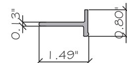
E23 SETTING CHAIR ES-WC25-011 ALUM. 6063-T6
