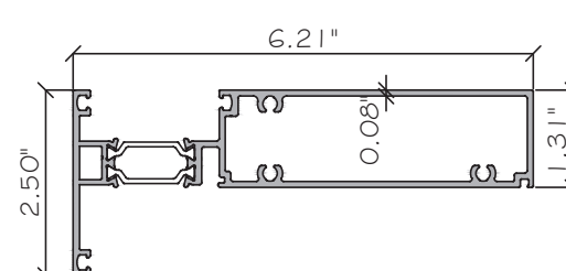
E4 INTERMEDIATE HORIZONTAL INSIDE ES-W625-G89 ALUM. 6063-T6
