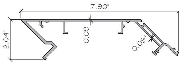
E17 OUTSIDE CORNER SSG-MALE ES-W625-025 ALUM. 6063-T6
