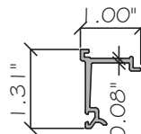
E22 INTERIOR GLASS STOP ES-WC25-009 ALUM. 6063-T6
