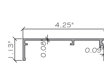
E10 MALE MULLION BACK ES-W625-002 ALUM. 6063-T6
