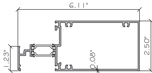
E3 INTERMEDIATE HORIZONTAL OUTSIDE ES-W625-G88 ALUM. 6063-T6
