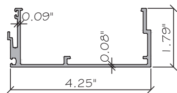
E11 SSG FEMALE MULLION ES-W625-003 ALUM. 6063-T6
