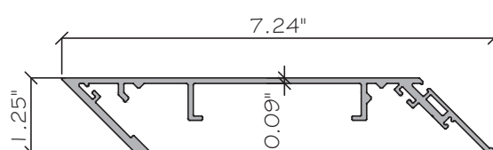
E18 OUTSIDE CORNER SSG-FEMALE ES-W625-026A ALUM. 6063-T6
