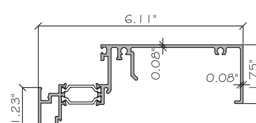
E5 SILL OUTSIDE ES-W625-G90 ALUM. 6063-T6
