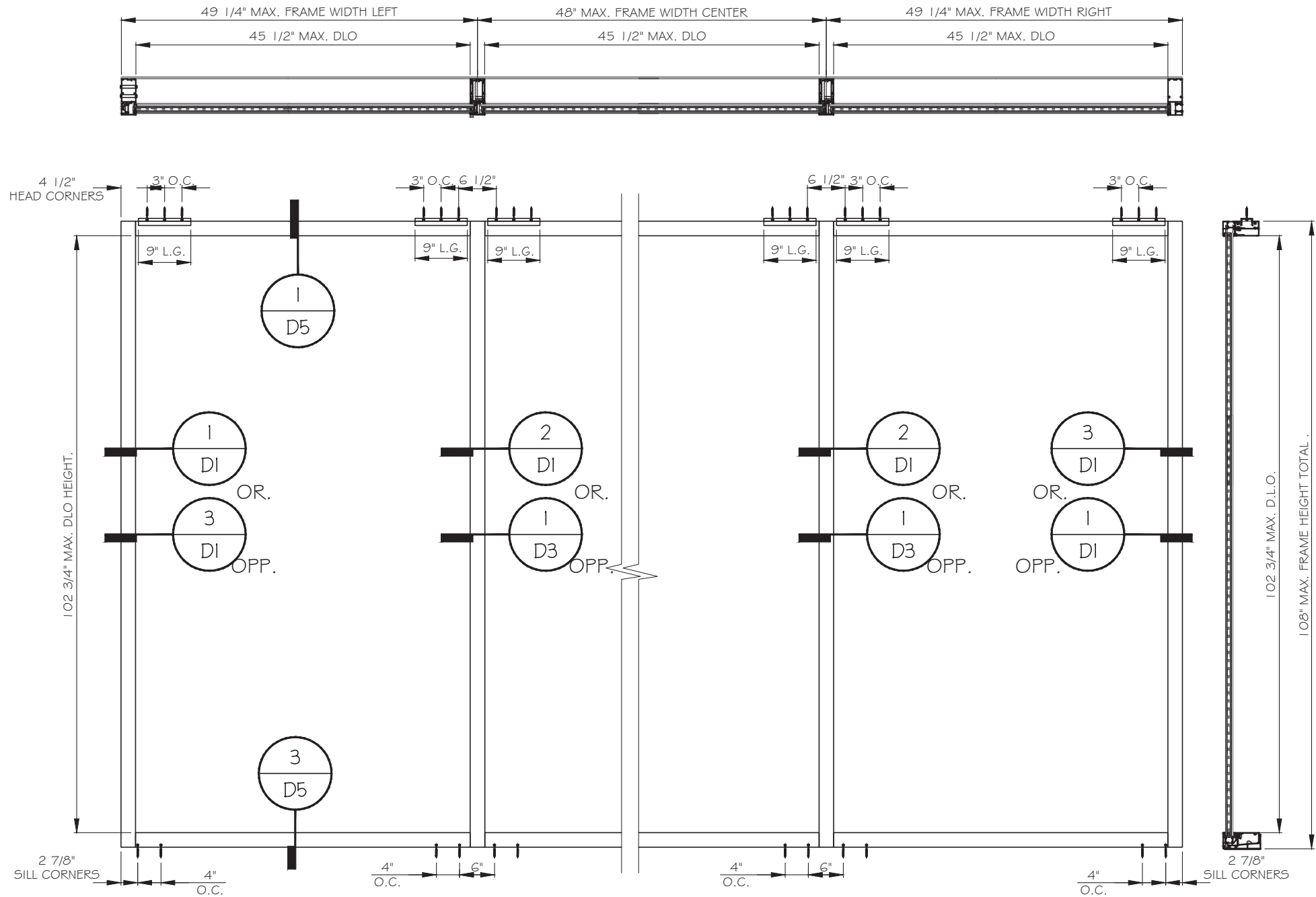
TYPICAL EXTERIOR ELEVATION (OUTSIDE RE-GLAZE) FOR SIZE SHOWN ABOVE OR SMALLER AS PERMITTED BY FBC.
