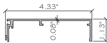
E12 SSG MALE MULLION ES-W625-004 ALUM. 6063-T6
