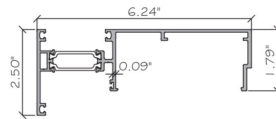
E9 VERTICAL MULLION ES-W625-G94 ALUM. 6063-T6
