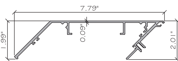
E20 INSIDE CORNER FEMALE ES-W625-028 ALUM. 6063-T6
