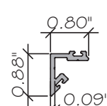
E21 INSIDE CORNER TRIM SSG ES-WC25-033 ALUM. 6063-T5
