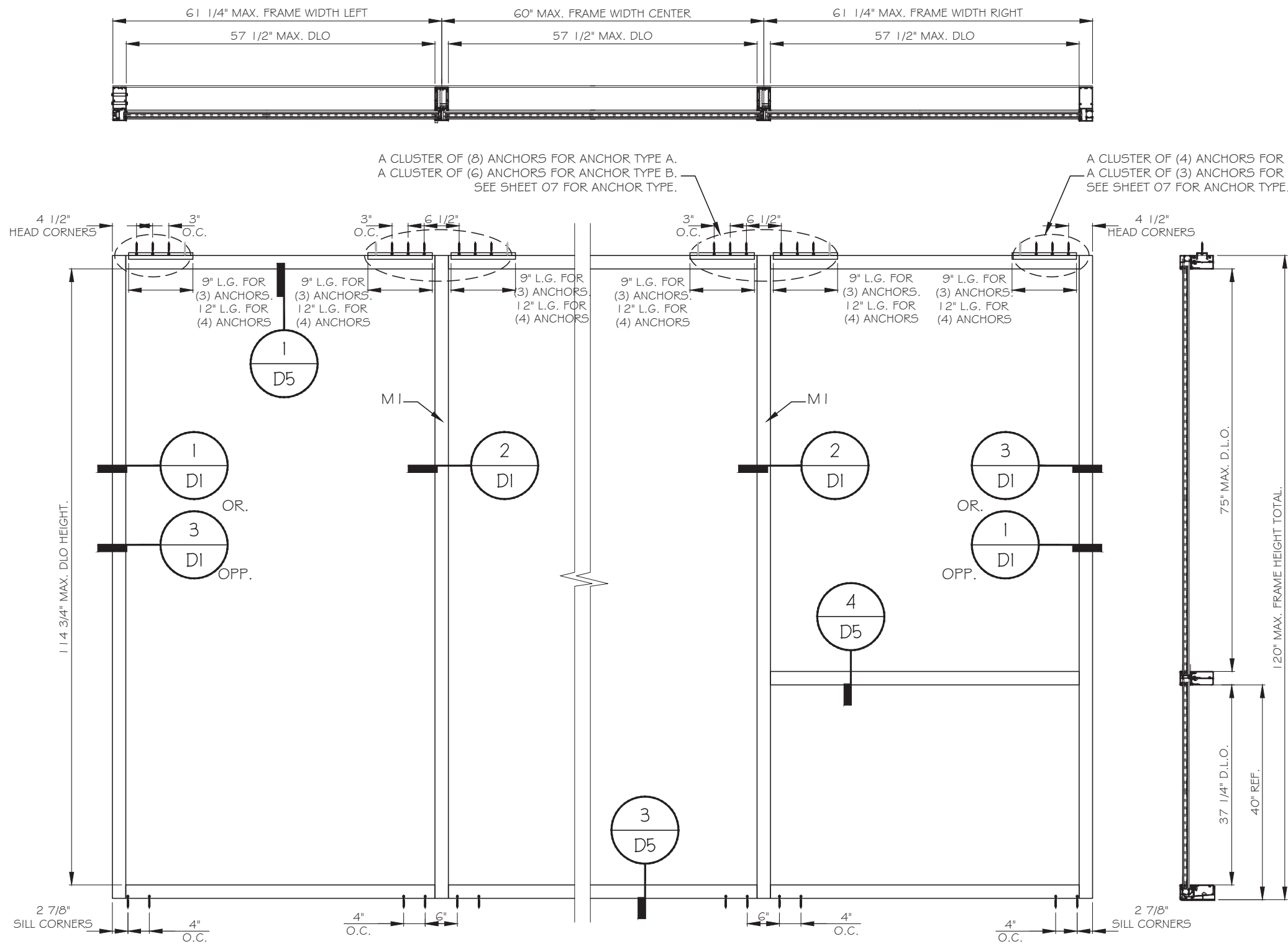
TYPICAL EXTERIOR ELEVATION (OUTSIDE RE-GLAZE) FOR SIZE SHOWN ABOVE OR SMALLER AS PERMITTED BY FBC. MAX. DESIGN LOAD: +/-65 PSF.
