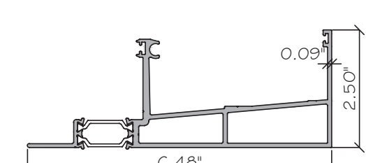
E7 STARTER SILL RECEPTOR ES-W625-G92 ALUM. 6063-T6
